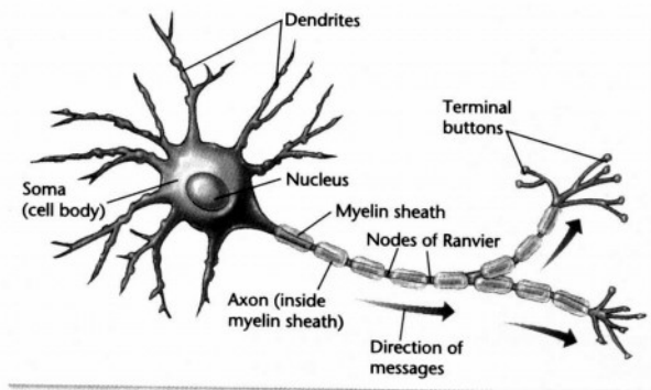
Figure 2-1 Schematic Diagram of a Neuron
