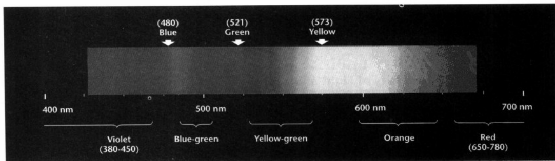
■ Figure 4-17 The Solar Spectrum
