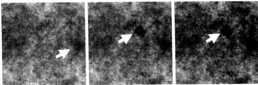
Figure 4-5 Examples of Signals Embedded in Noise
