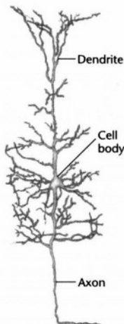
Figure 2-3 Shapes and Relative Sizes of Neurons
