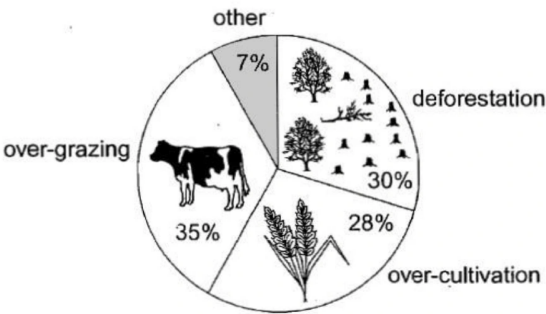
Causes of worldwide land degradation
