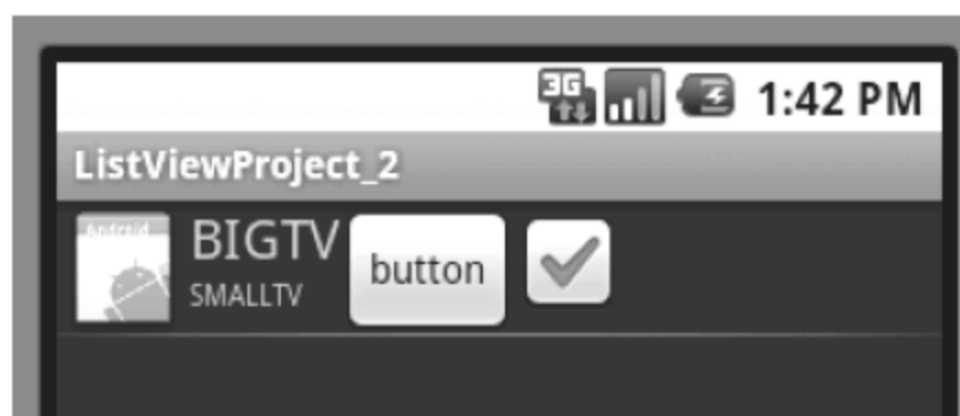
图 3-36 ListView (SimpleAdapter)
