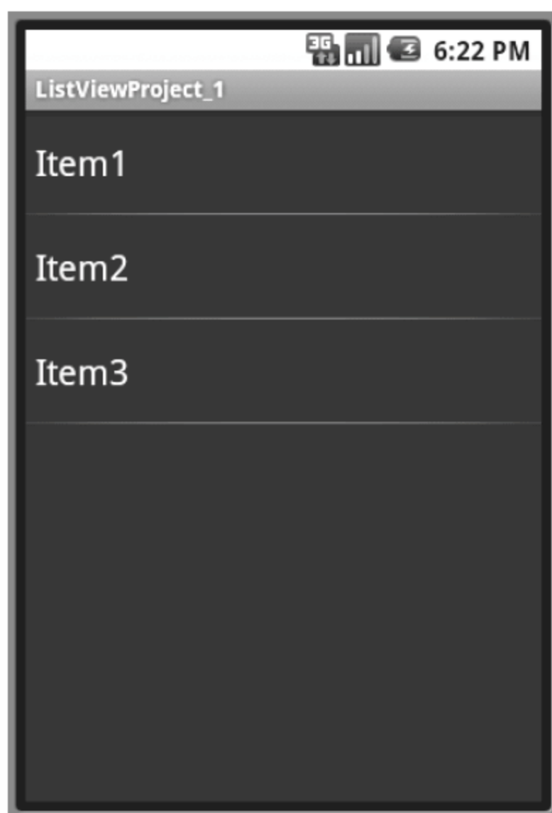
图 3-35 ListView (ArrayAdapter)
